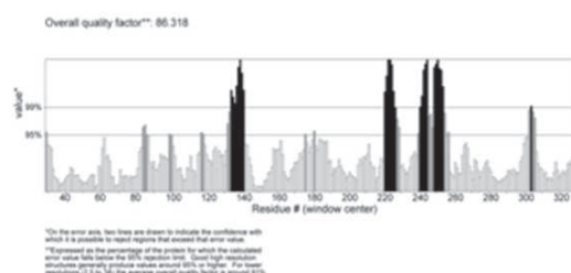
Figure 6: Errat analysis data of human GRIN 1 protein.
