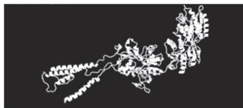
Figure 2: Figure showing the modeled structure of human GRIN 1 protein
