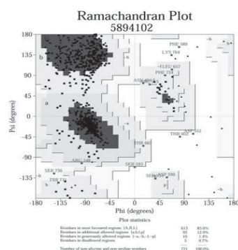
Figure 5: Ramachandran plot analysis data of GRIN 1 Protein
