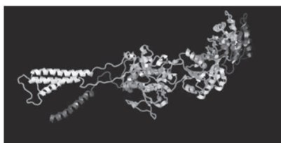
Figure 4: Three dimensional arrangement of different secondary structures in the modeled human GRIN1 proteins
